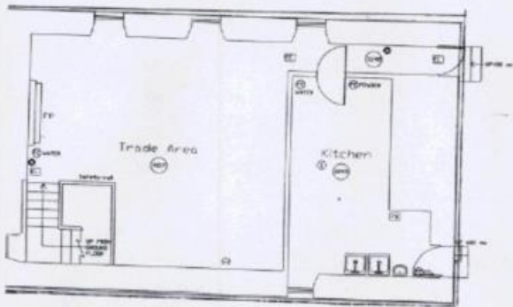
SCALE 1:100 FIRST FLOOR
