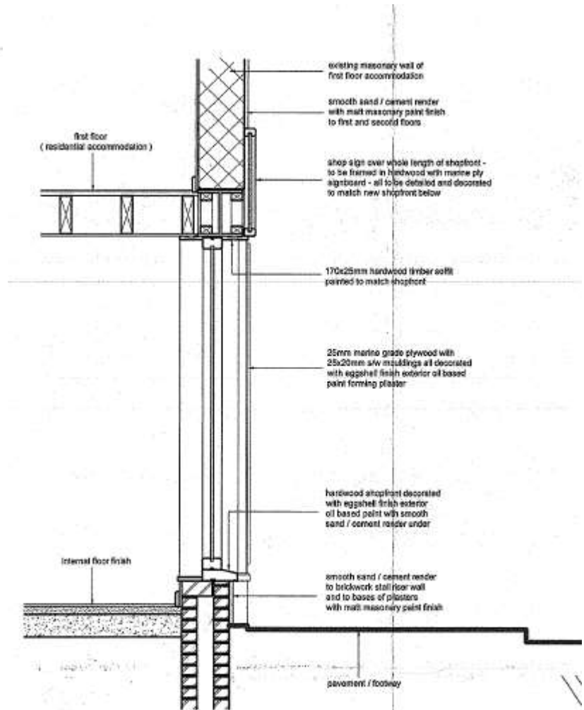
Proposed section AA through shopfront 1:20 Toriad arfaethedig AA drwy ffrynt y siop 1:20
